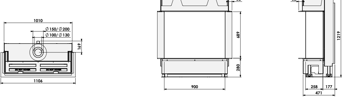
Gas Fire Panorama 110-70
