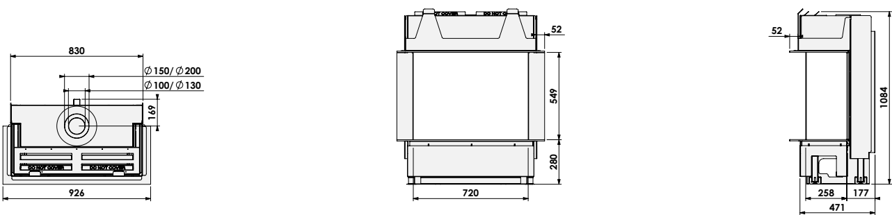
Gas Fire Panorama 90-55
